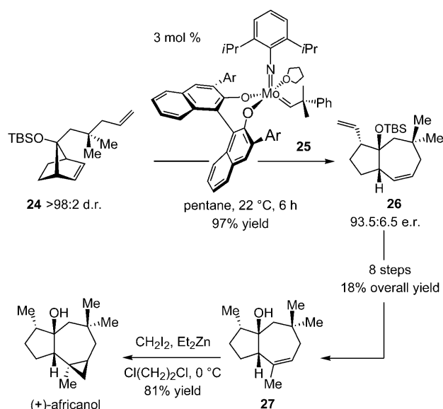
Scheme 7. Synthesis of africanol through an enantioselective ring-opening/ring-closing metathesis (RORCM) reaction. Ar = 2,4,6-( i Pr) 3 C 6 H 2 , TBS = tert -butyldimethylsilyl.
