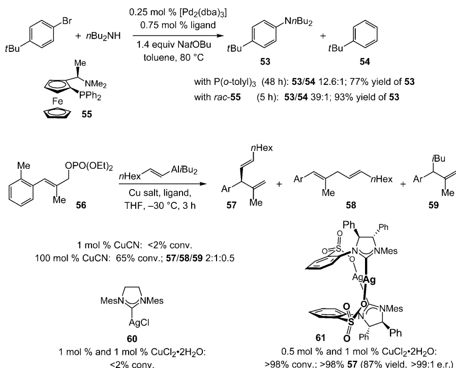
Scheme 14. Chiral Pd- and Cu-based complexes generate product-selectivity, site-selectivity and efficiency levels that are superior to those afforded by the corresponding achiral catalysts.
