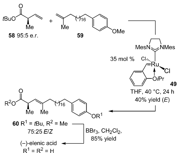
Scheme 15. Natural product synthesis often underlines significant deficiencies in catalyst development, as indicated by an inefficient cross-metathesis reaction in an enantioselective synthesis of elenic acid.
