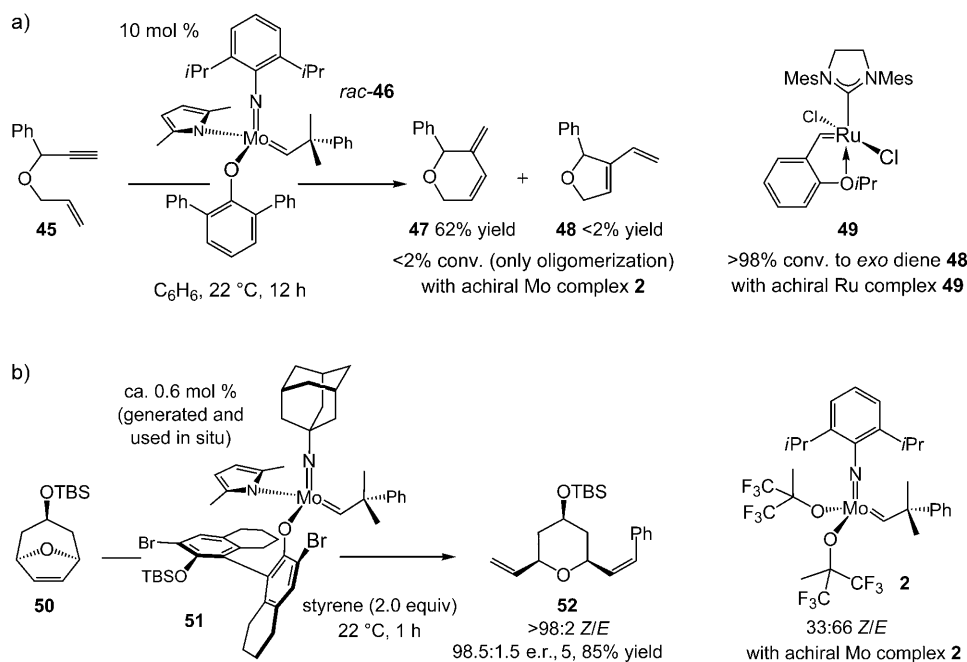
Scheme 13. Chiral olefin metathesis catalysts are not only valuable for obtaining enantiomerically enriched products; they can also offer other types of selectivity. Mes = 2,4,6-Me 3 -C 6 H 2 .
