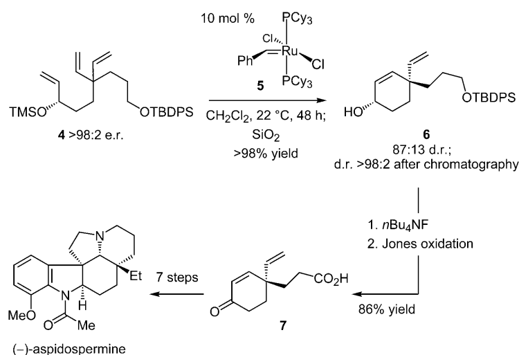
Scheme 2. Total synthesis of aspidospermine through catalytic diastereoselective RCM. TMS = trimethylsilyl; TBDPS = tert -butyldiphenylsilyl.
