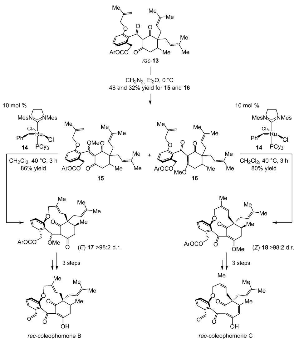
Scheme 4. Control of atropisomerism in total syntheses of rac -coleophomones B and C. Ar = p\text{BrC}_6\text{H}_4 ; Mes = 2,4,6- \text{Me}_3\text{C}_6\text{H}_2 .
