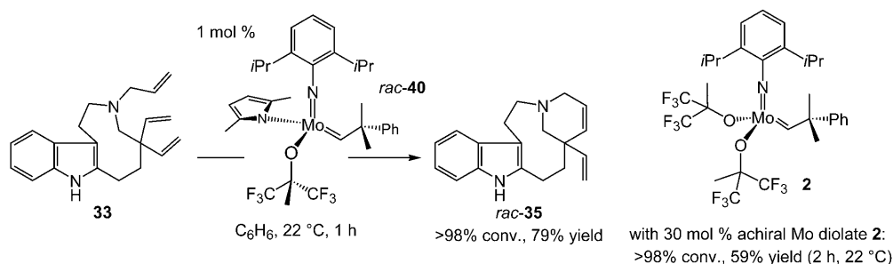
Scheme 11. A stereogenic-at-Mo complex serving as a uniquely efficient RCM catalyst.
