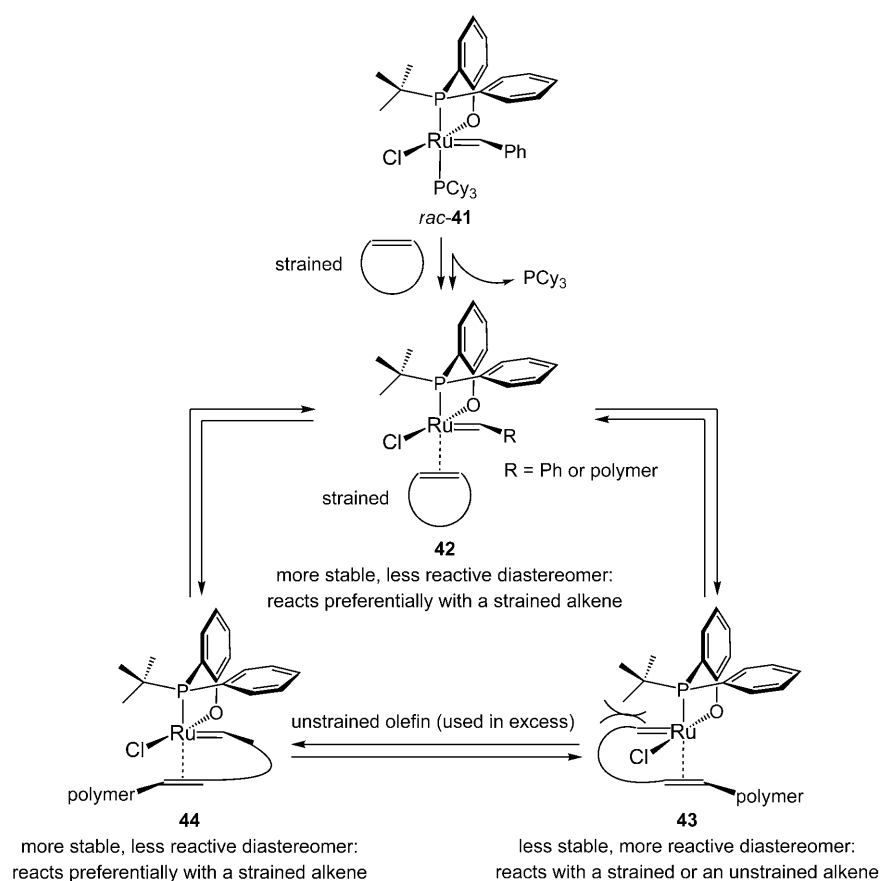
Scheme 12. A racemic stereogenic-at-Ru catalyst used to promote sequence-selective polymerization; success of this strategy is due to energy differences between the two carbene diastereomers of the chiral complex.
