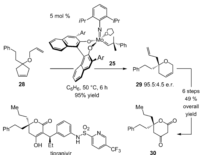
Scheme 8. Enantioselective synthesis of the lactone fragment of HIV-protease inhibitor tipranivir through a Mo-catalyzed ring-opening/ring-closing metathesis (RORCM) reaction. Ar = 2,4,6- i Pr 3 C 6 H 2 .
