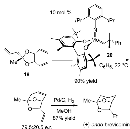
Scheme 5. Synthesis of (+)-endo-brevicomin through enantioselective RCM.
