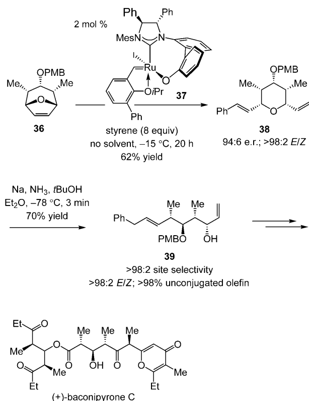
Scheme 10. Total synthesis of baconipyrrone C through an enantioselective Ru-catalyzed ring-opening/cross-metathesis (ROCM) reaction. PMB = p -methoxybenzyl; Mes = 2,4,6-Me 3 C 6 H 2 .
