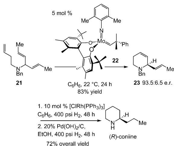
Scheme 6. Total synthesis of coniine through enantioselective RCM.
