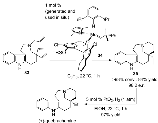
Scheme 9. Catalyst development spurred by total synthesis: A stereogenic-at-Mo complex as a highly effective chiral catalyst developed for enantioselective RCM in total synthesis of quebrachamine. TBS = tert -butyldimethylsilyl.
