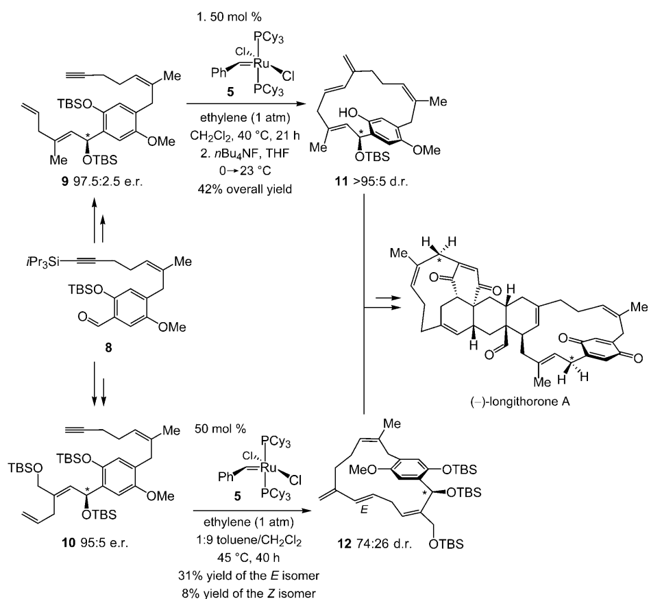
Scheme 3. Total synthesis of (-)-longithorone A involving a diastereoselective enyne RCM. The silyl ether-bearing stereogenic carbon centers, installed for control of planar stereogenicity and subsequently removed, are highlighted. TBS = tert -butyldimethylsilyl.
